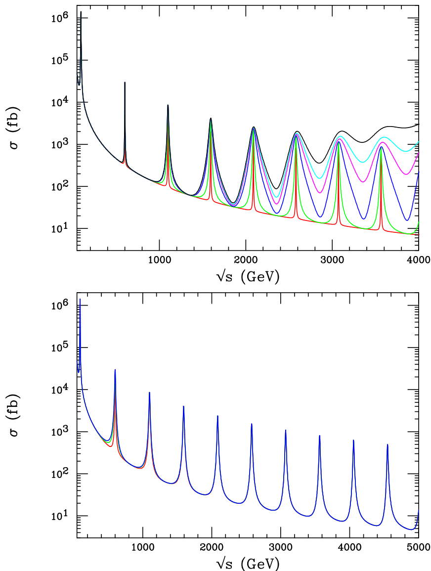
Figure 12: Cross section for e^+e^- \rightarrow \mu^+\mu^- as a function of \sqrt{s} in the RS model with c = 0.05 and m_1 = 600 \text{ GeV} showing the first 7(9) graviton KK excitations in the top(bottom) panel. In the top panel, the uppermost curve corresponds to the standard result. Moving inward the curves correspond to the case where a form factor is present assuming t = 4(3, 2, 1, 0.5) , respectively. In the lower panel, t = 1 has been assumed for very large values of c = 0.1, 0.2 and 0.3 , with the narrowest resonance curve corresponding to the smallest value of c .
