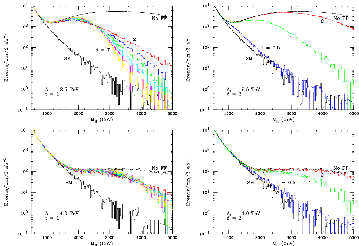
Figure 3: The event rate per bin with 3 \text{ ab}^{-1} of integrated luminosity for Drell-Yan production at the LHC as a function of the lepton pair invariant mass taking the scale \Lambda_H = 2.5 \text{ TeV} (top panels) and \Lambda_H = 4.0 \text{ TeV} (bottom panels). In the left panels, t = 1 and \delta = 2, 3, 4, 5, 6, 7 from top to bottom on the right-hand side as labeled. In the right panels, \delta = 3 and the red, green, blue curves correspond to t = 2, 1, 0.5 . In all panels, the bottom black histogram corresponds to the Standard Model result, and the top black histogram is the conventional ADD result [20] without the form factor.
