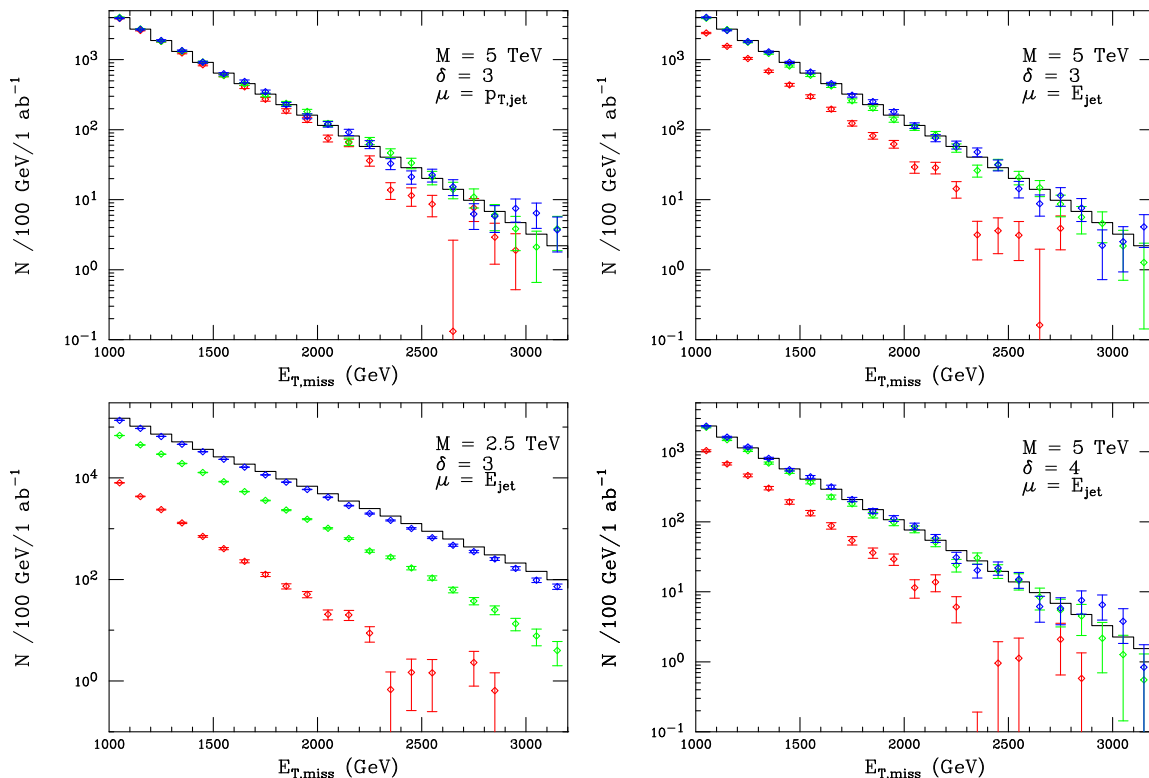
Figure 5: Missing transverse energy distribution for the signal process pp \rightarrow jet + \cancel{E}_T assuming 1 \text{ ab}^{-1} of integrated luminosity at the LHC. The standard ADD result is given by the black histogram, while the blue, green, and red data points correspond to the inclusion of the form factor with t = 2, 1, 0.5 , respectively. The other parameters are as labeled. The errors bars represent the statistical errors.
